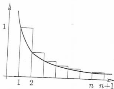
Steps above the function f(t) = \frac{1}{t}
