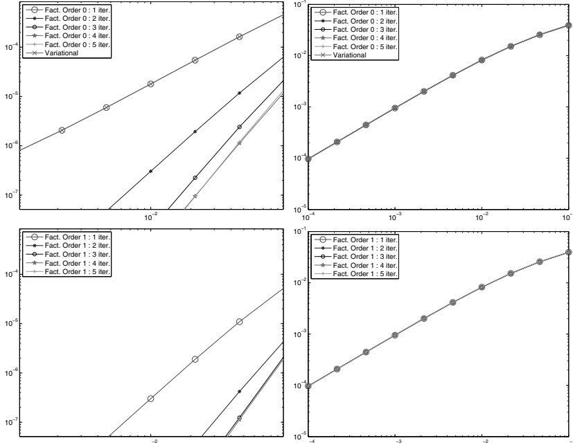
Fig. 1. Positive advection. Factorization method of order 0 and variational method (4) in the top row , and first order method in the bottom row . Error versus viscosity on (-L_1, 0) on the left , and on (0, L_2) on the right .
